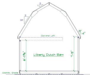
DUTCH LIBERTY GARAGE
