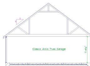
CLASSIC GARAGE ATTIC TRUSS
