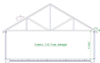
CLASSIC GARAGE 7/12 TRUSS
