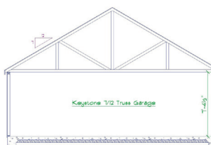
KEYSTONE GARAGE 7/12 TRUSS
