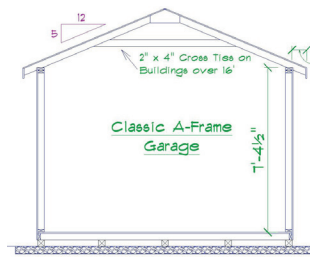
CLASSIC A-FRAME GARAGE
