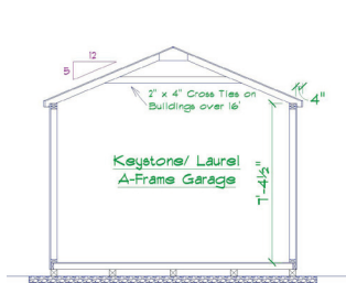
KEYSTONE & LAUREL A-FRAME GARAGE
